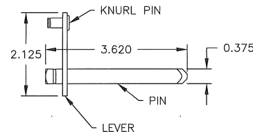
54 DAMPER AXLE ASSEMBLY, DRIVE SIDE MATERIAL VARIES
