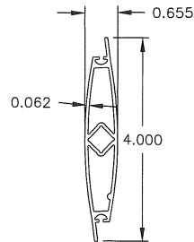
47 DAMPER BLADE 6063-T5 ALUMINUM
