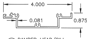
45 DAMPER HEAD/SILL 6063-T5 ALUMINUM
