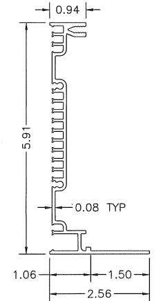
⑧ JAMB (SLEEVE FRAME) 6005-T5 ALUMINUM
