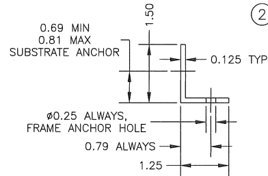
⑤ MOUNTING ANGLE (CHANNEL FRAME) 6061-T6 ALUMINUM
