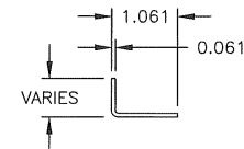
50 DAMPER TOP/BOTTOM CLOSURE ALUMINUM
