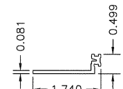
44 DAMPER FLANGE 6063-T5 ALUMINUM
