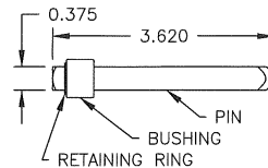
53 DAMPER AXLE ASSEMBLY, NON-DRIVE SIDE MATERIAL VARIES
